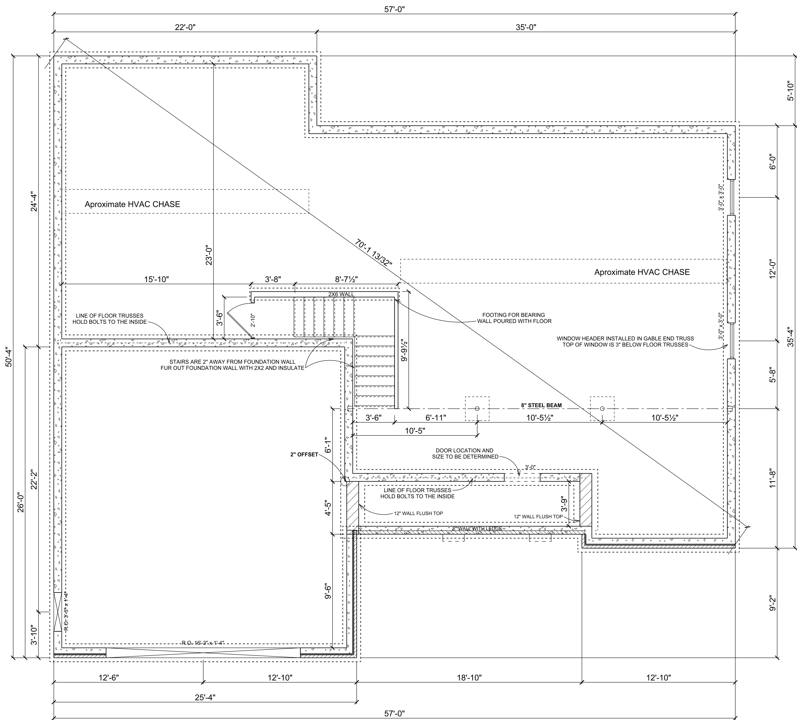
FOUNDATION LAYOUT
